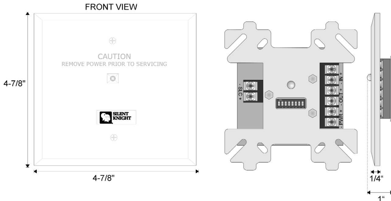
Model SD500-ANM Addressable Notification Module
